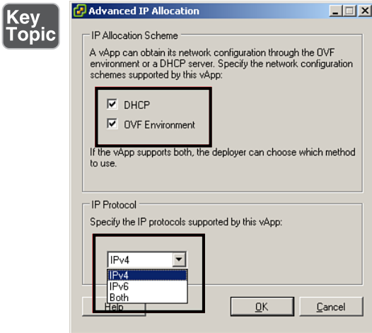
Figure 4-31 Advanced IP Allocation Settings for vApps
