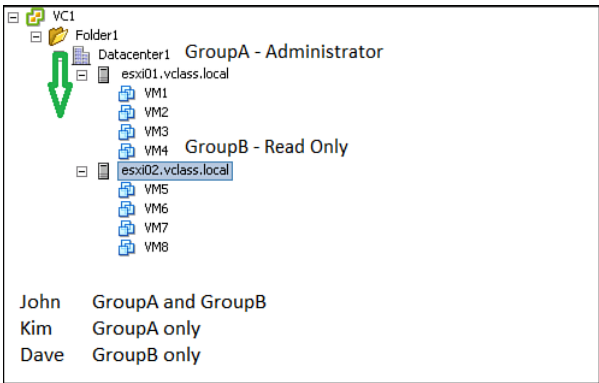
Figure 1-29 Direct Permissions on Groups Supersede Inherited
