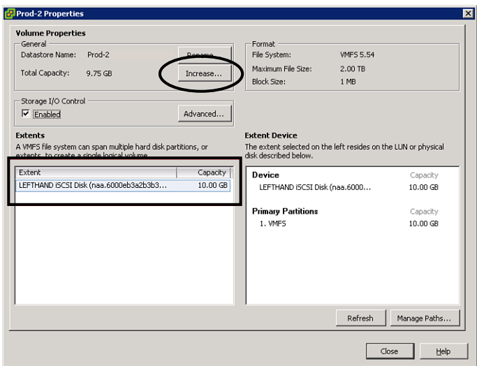
Figure 3-47 Viewing Datastore Extents
