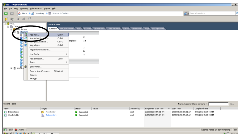
Figure 5-3 Adding a Host to a Cluster
