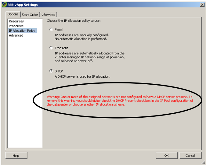
Figure 4-29 Configuring DHCP Settings for vApps
