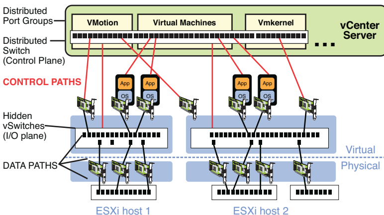
Figure 2-37 Distributed Switch Architecture
