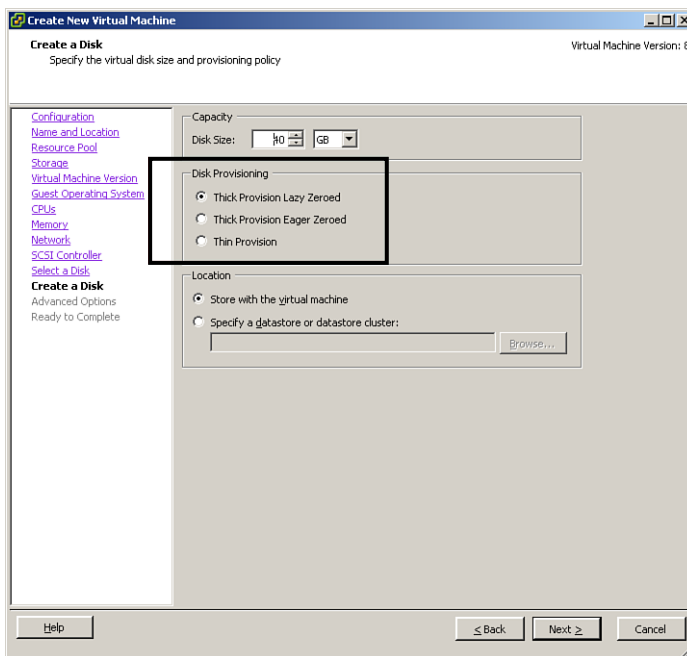
Figure 4-8 Virtual Disk Provisioning
