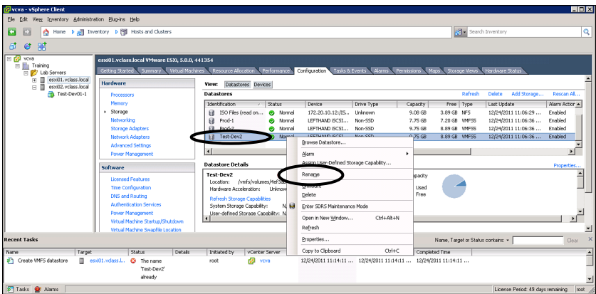
Figure 3-35 Selecting a Datastore to Rename
