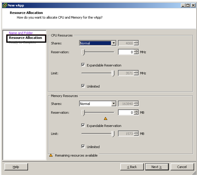
Figure 4-35 The Resource Allocation Page
