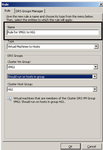
Figure 5-29 Creating a DRS Group - Adding Rules
