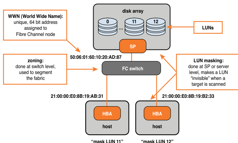
Figure 3-6 Zoning and Masking
