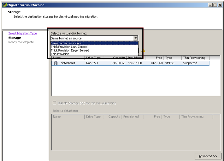
Figure 5-62 Changing Disk Format During Storage vMotion
