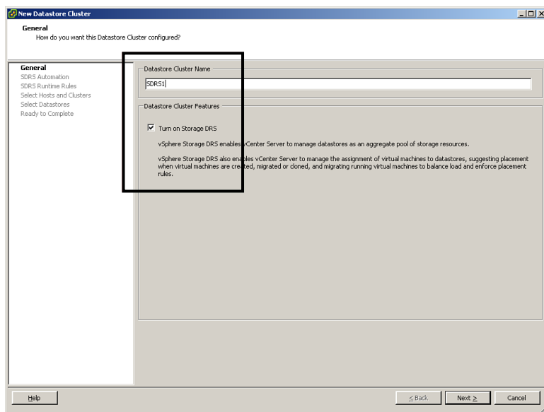
Figure 5-14 Enabling SDRS in a Datastore Cluster
