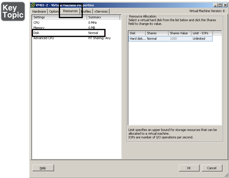
Figure 4-10 Configuring Disk Resources
