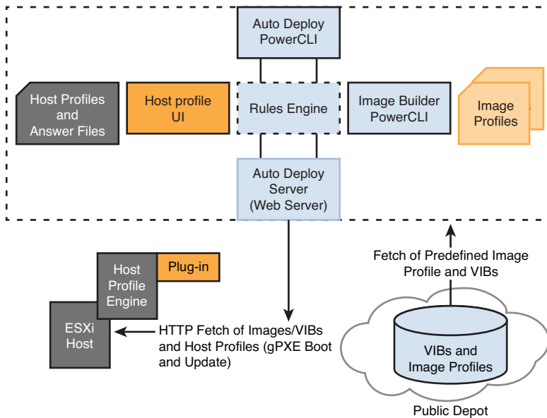
Figure 1-11 Auto Deploy Architecture
