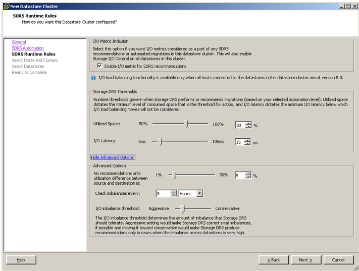
Figure 5-16 Configuring SDRS Runtime Rules
