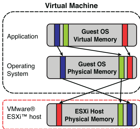
Figure 7-5 The Memory “Shell Game”
