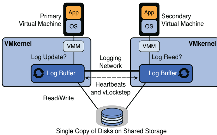
Figure 5-36 vSphere FT Architecture
