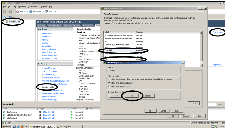
Figure 6-6 Configuring the ESXi Shell and SSH Services
