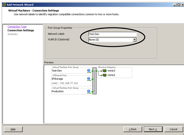
Figure 2-21 Entering and Network Label
