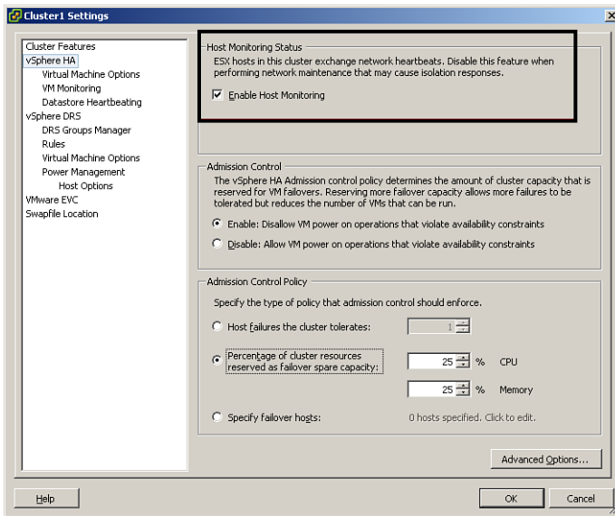
Figure 5-31 Enabling/Disabling Host Monitoring
