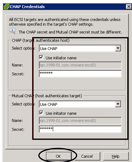
Figure 3-22 Configuring Mutual CHAP
