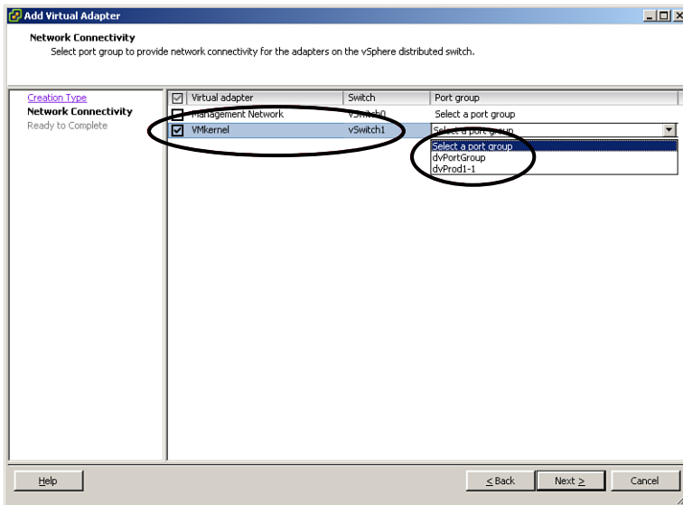
Figure 2-52 Choosing a Port Group
