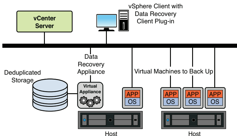
Figure 5-72 VDR at a Glance
